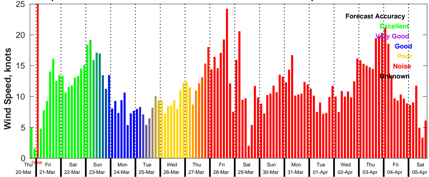
GFS Wind Speed Forecast for NDBC 42019 from 20-Mar-2025 18:00:00 to 05-Apr-2025 18:00:00
