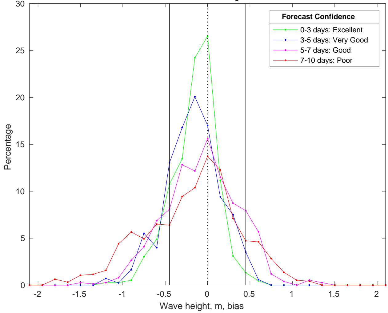
NDBC 42020 vs CMEMS Waves Bias Histogram: 21-Mar-2025
