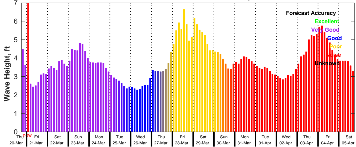
GFS Wave Forecast for NDBC 42020 from 20-Mar-2025 18:00:00 to 05-Apr-2025 18:00:00
