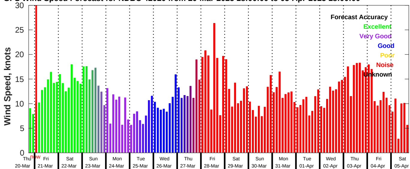
GFS Wind Speed Forecast for NDBC 42020 from 20-Mar-2025 18:00:00 to 05-Apr-2025 18:00:00
