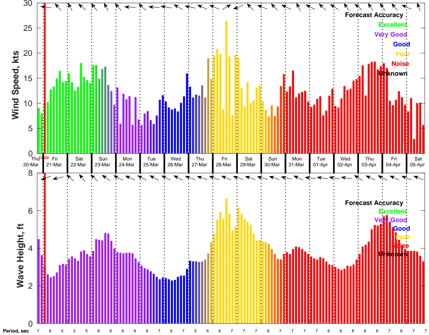
Wind & Wave Forecast for NDBC 42020 from 20-Mar-2025 18:00:00 to 05-Apr-2025 18:00:00
