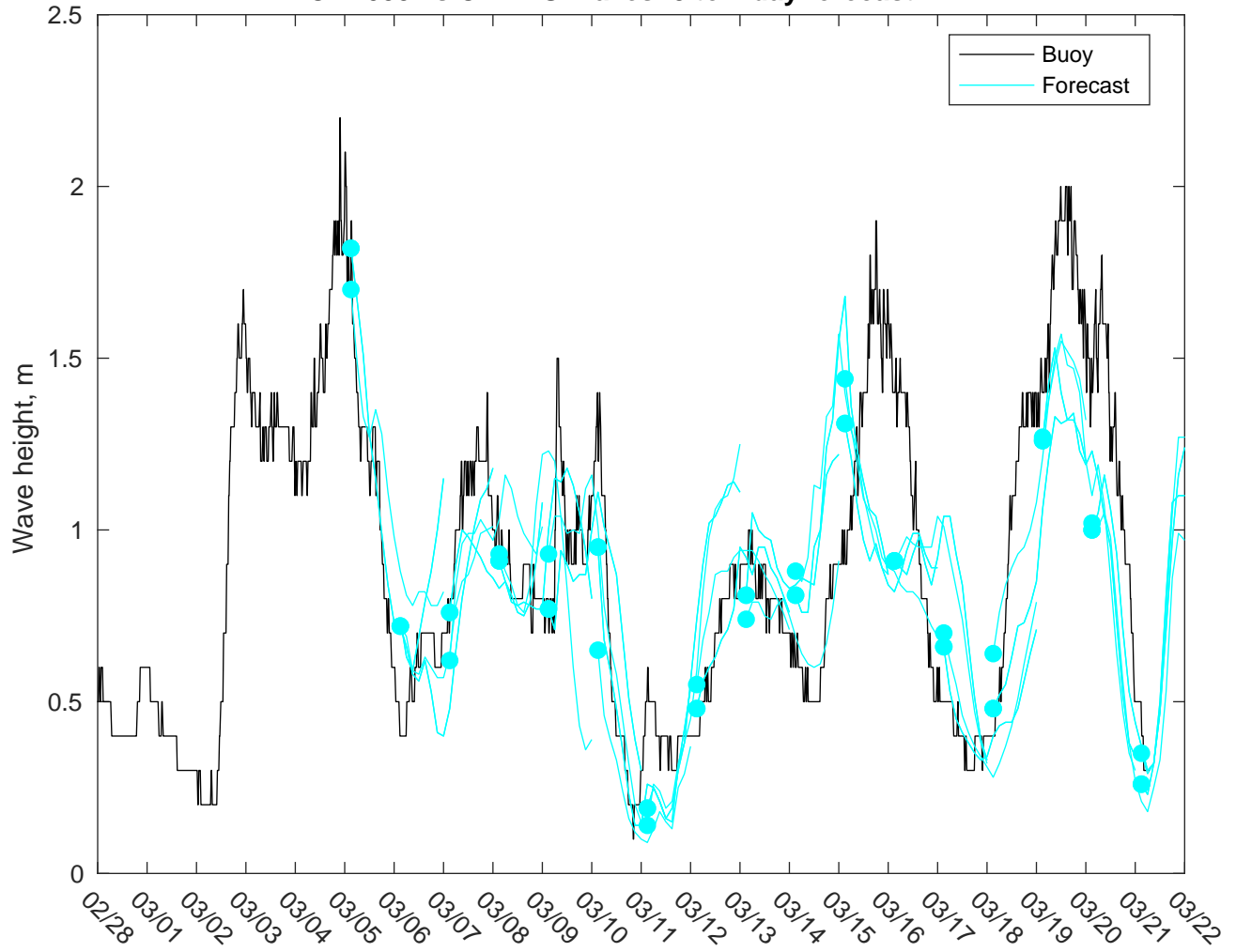
NDBC 42035 vs CMEMS Waves: 5 to 7 day forecast
