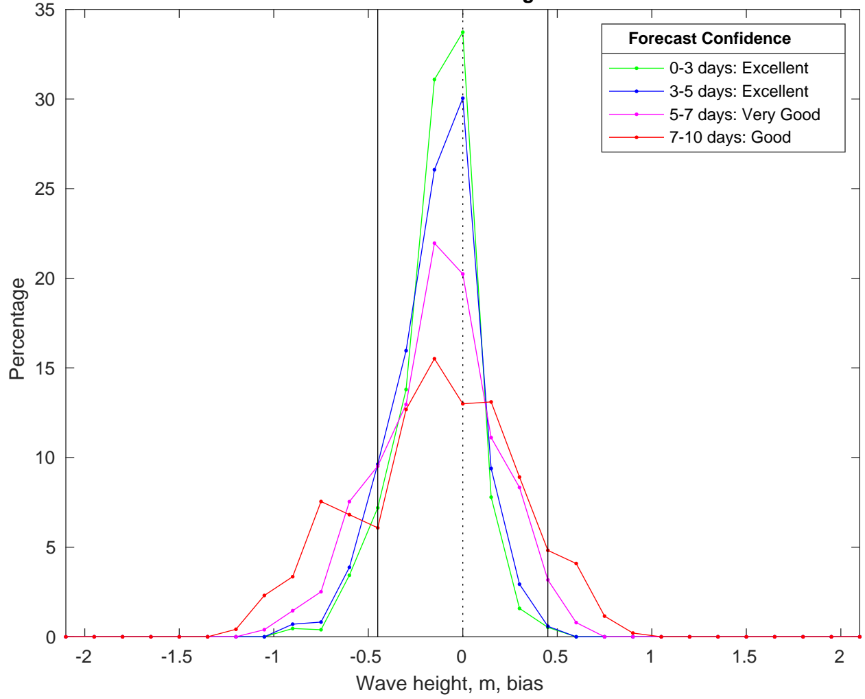
NDBC 42035 vs CMEMS Waves Bias Histogram: 21-Mar-2025
