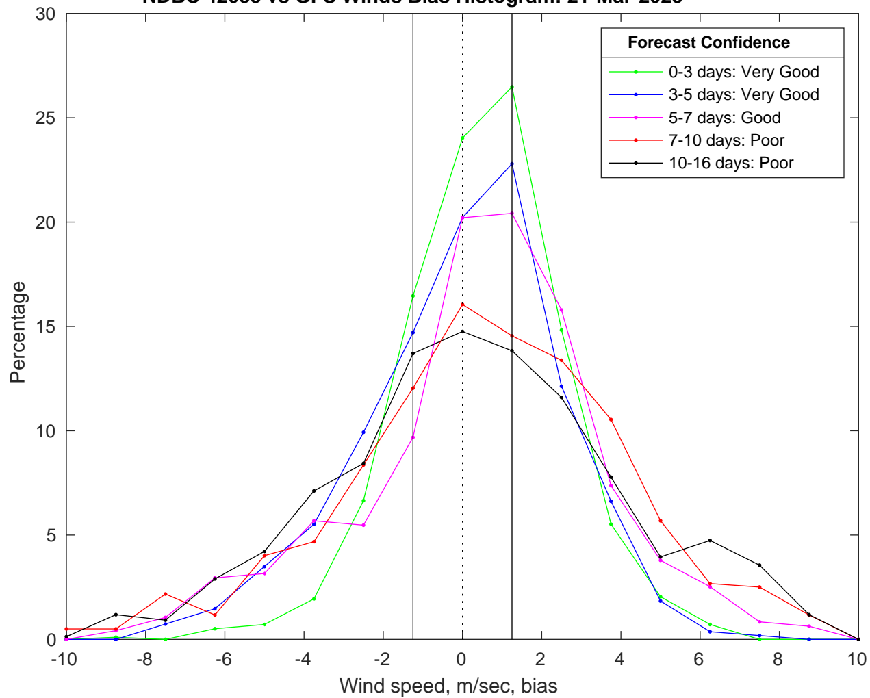
NDBC 42035 vs GFS Winds Bias Histogram: 21-Mar-2025
