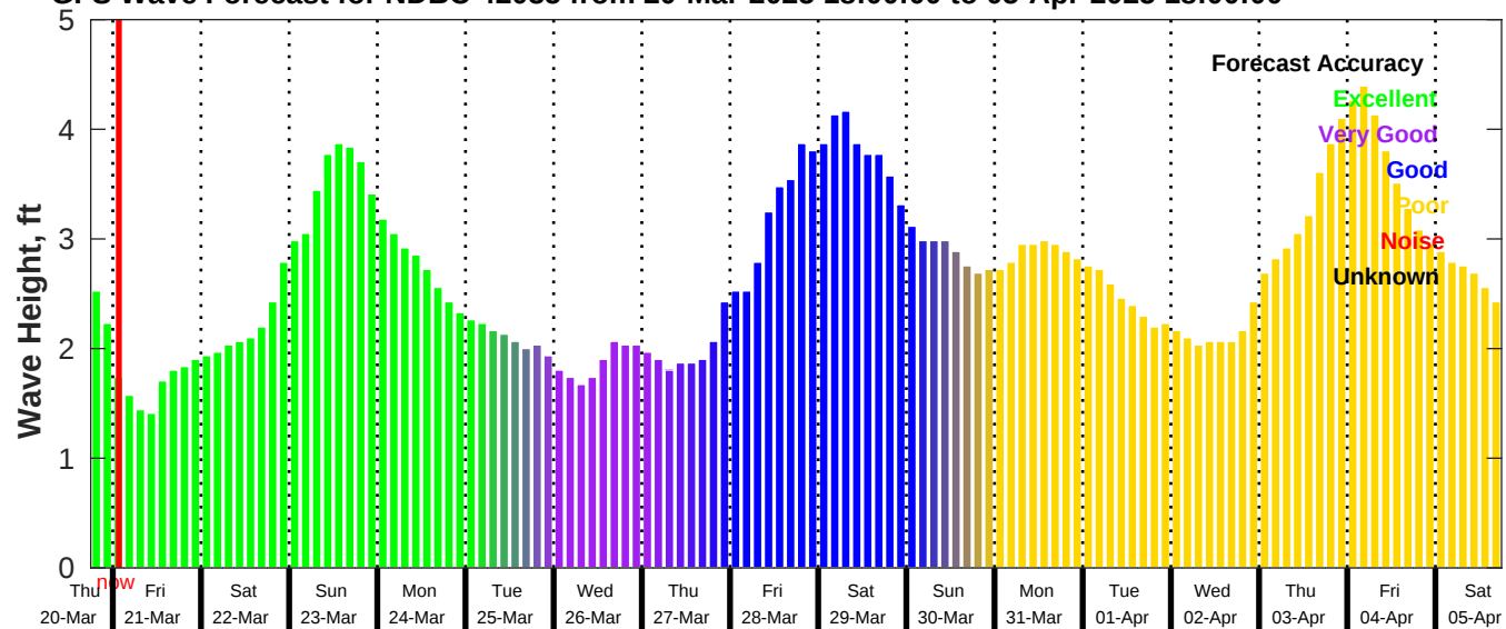
GFS Wave Forecast for NDBC 42035 from 20-Mar-2025 18:00:00 to 05-Apr-2025 18:00:00
