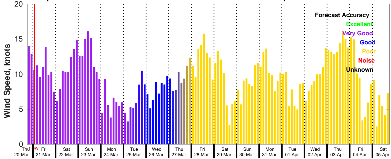
GFS Wind Speed Forecast for NDBC 42035 from 20-Mar-2025 18:00:00 to 05-Apr-2025 18:00:00
