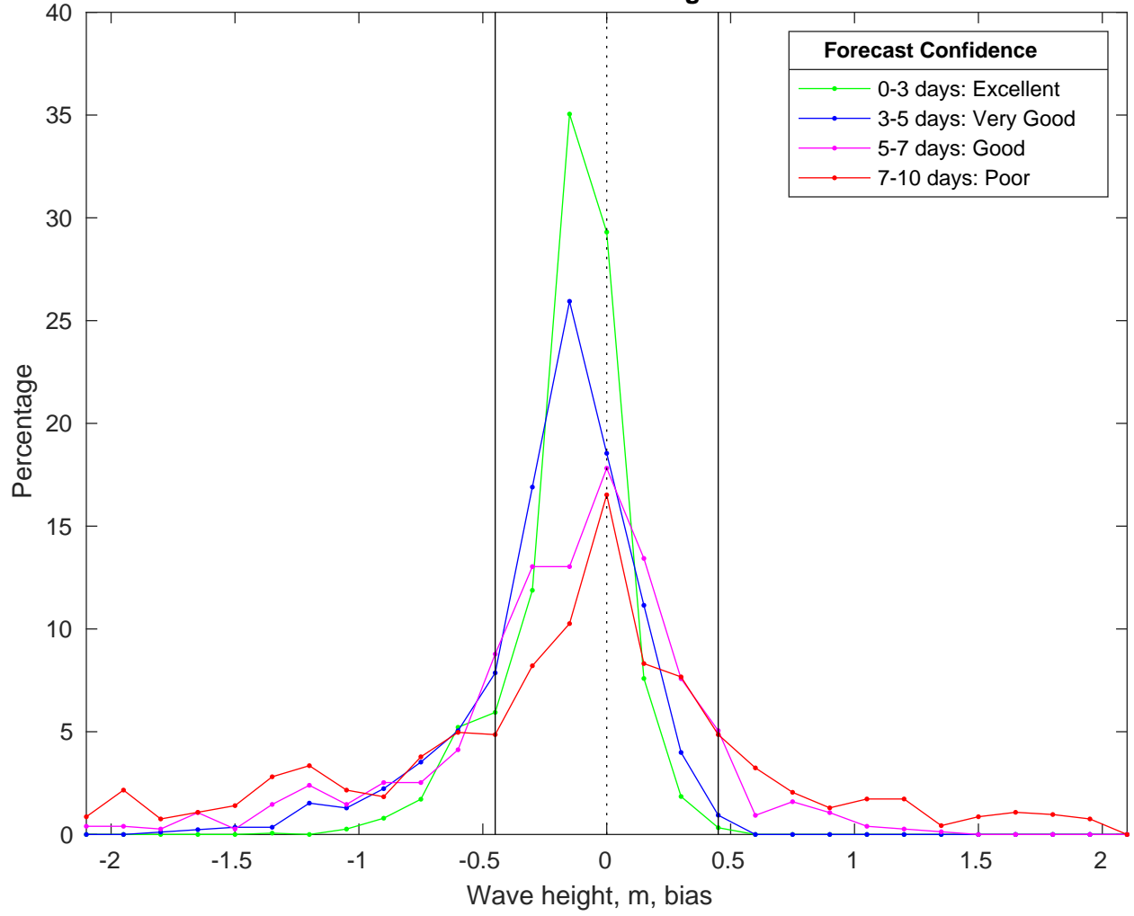
NDBC 42036 vs CMEMS Waves Bias Histogram: 21-Mar-2025
