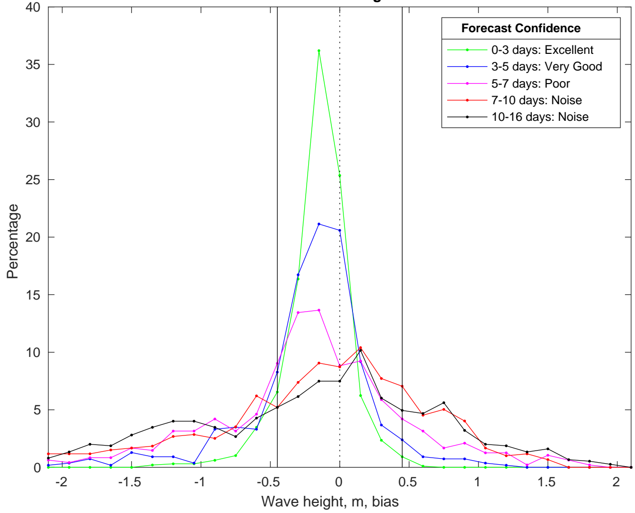
NDBC 42036 vs GFS Waves Bias Histogram: 21-Mar-2025
