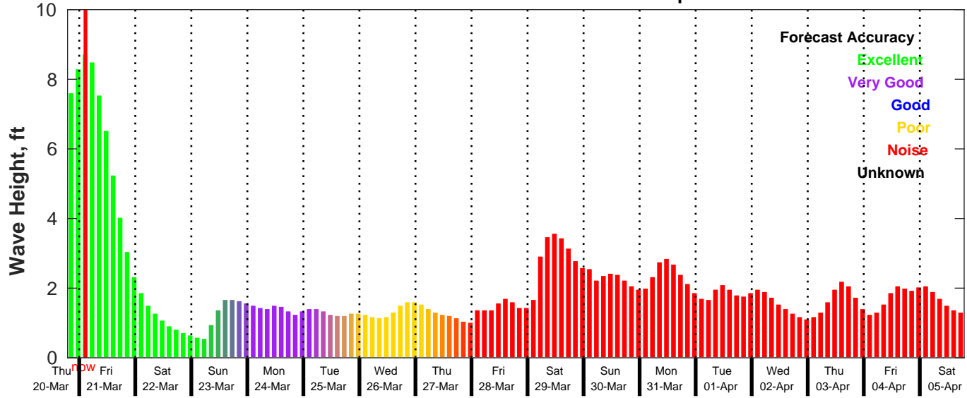
GFS Wave Forecast for NDBC 42036 from 20-Mar-2025 19:00:00 to 05-Apr-2025 19:00:00
