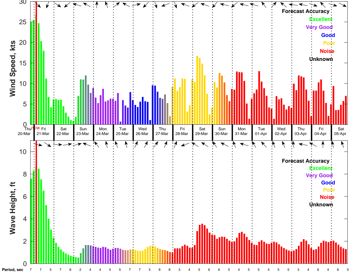
Wind & Wave Forecast for NDBC 42036 from 20-Mar-2025 19:00:00 to 05-Apr-2025 19:00:00
