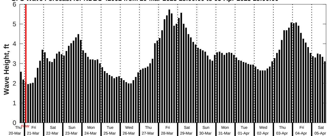
GFS Wave Forecast for NDBC 42092 from 20-Mar-2025 18:00:00 to 05-Apr-2025 18:00:00
