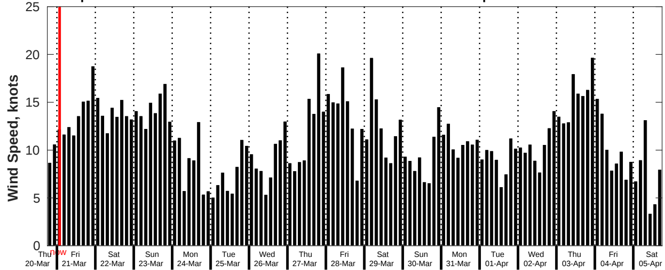
GFS Wind Speed Forecast for NDBC 42092 from 20-Mar-2025 18:00:00 to 05-Apr-2025 18:00:00
