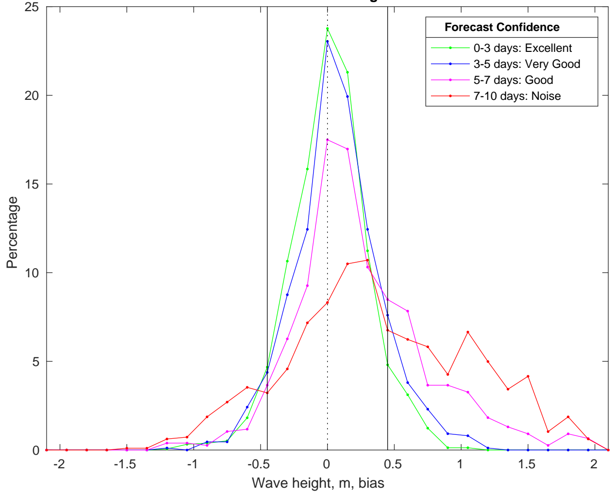
NDBC 46011 vs CMEMS Waves Bias Histogram: 21-Mar-2025
