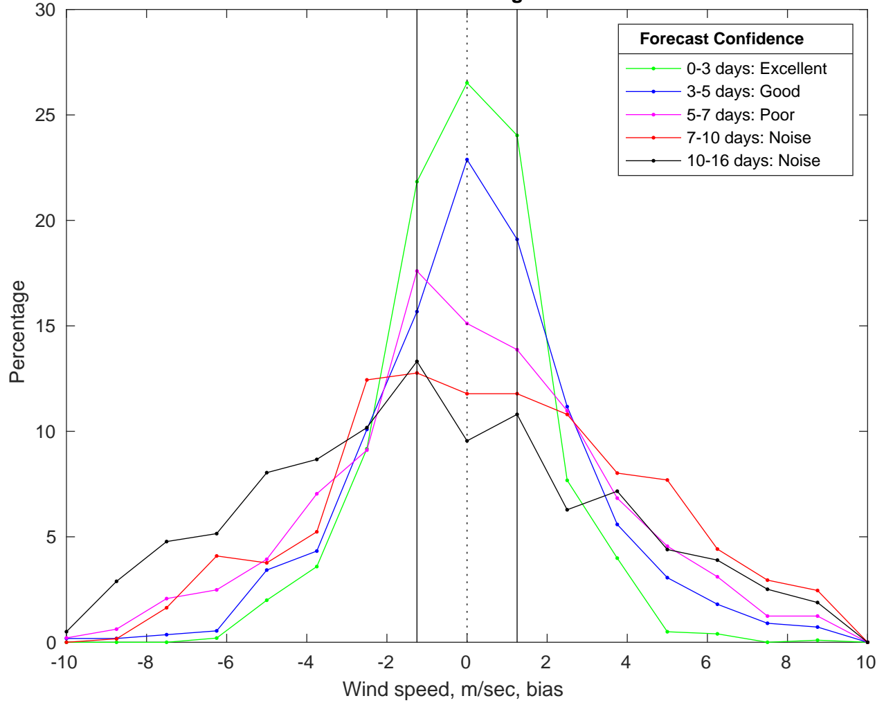
NDBC 46011 vs GFS Winds Bias Histogram: 21-Mar-2025
