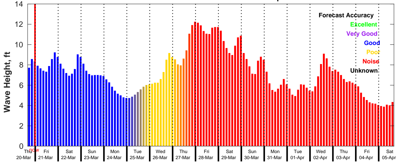
GFS Wave Forecast for NDBC 46011 from 20-Mar-2025 16:00:00 to 05-Apr-2025 16:00:00
