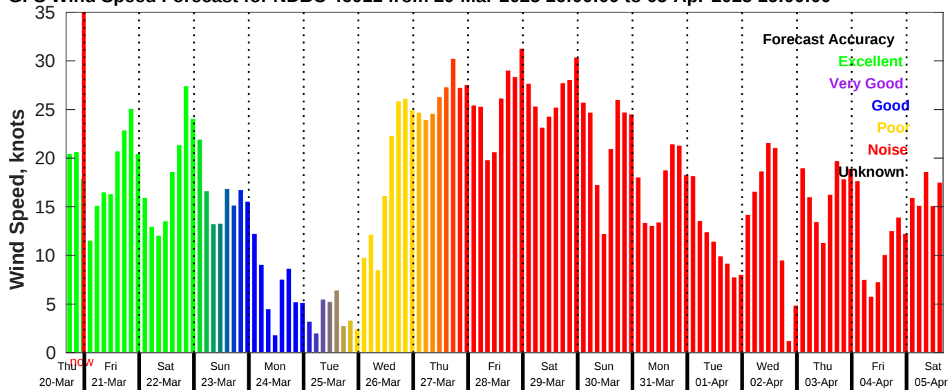
GFS Wind Speed Forecast for NDBC 46011 from 20-Mar-2025 16:00:00 to 05-Apr-2025 16:00:00
