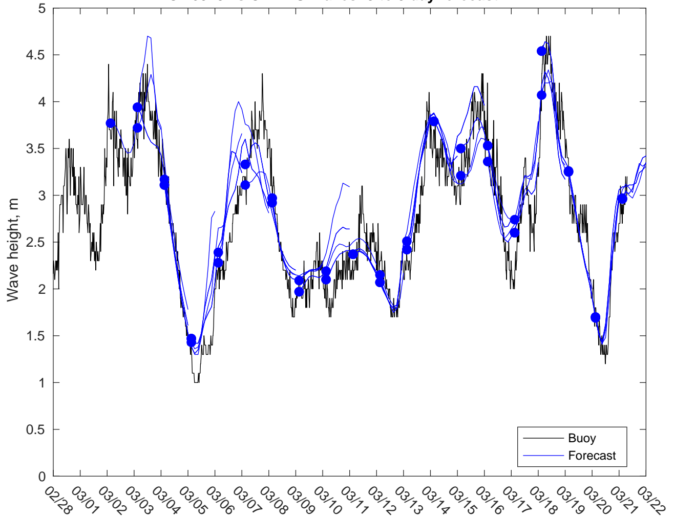
NDBC 46028 vs CMEMS Waves: 3 to 5 day forecast
