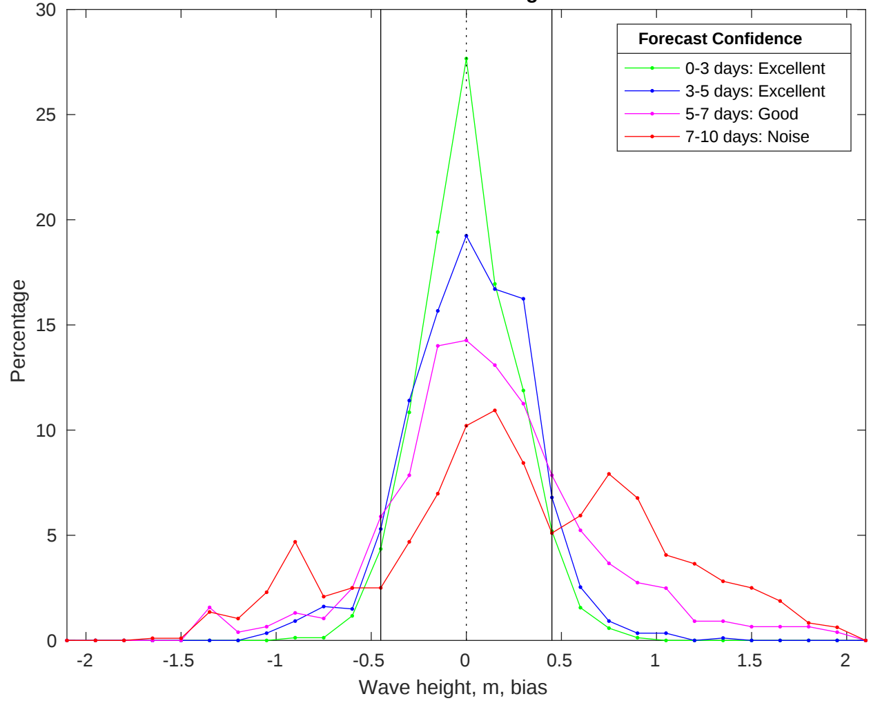
NDBC 46028 vs CMEMS Waves Bias Histogram: 21-Mar-2025
