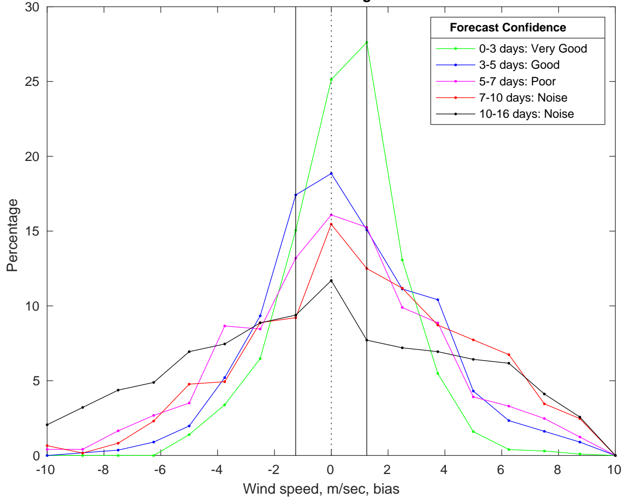
NDBC 46028 vs GFS Winds Bias Histogram: 21-Mar-2025
