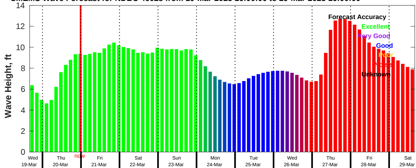
CMEMS Wave Forecast for NDBC 46028 from 19-Mar-2025 16:00:00 to 29-Mar-2025 16:00:00
