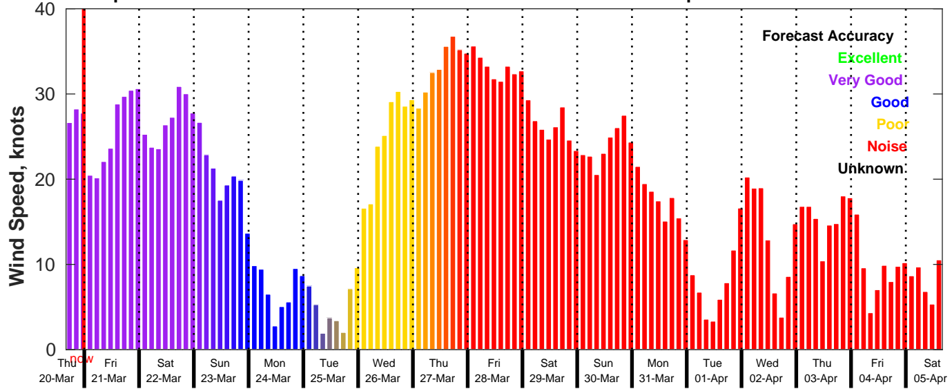
GFS Wind Speed Forecast for NDBC 46028 from 20-Mar-2025 16:00:00 to 05-Apr-2025 16:00:00
