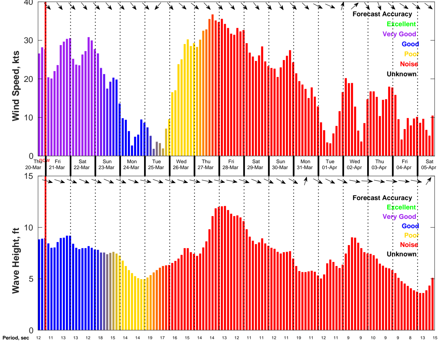
Wind & Wave Forecast for NDBC 46028 from 20-Mar-2025 16:00:00 to 05-Apr-2025 16:00:00
