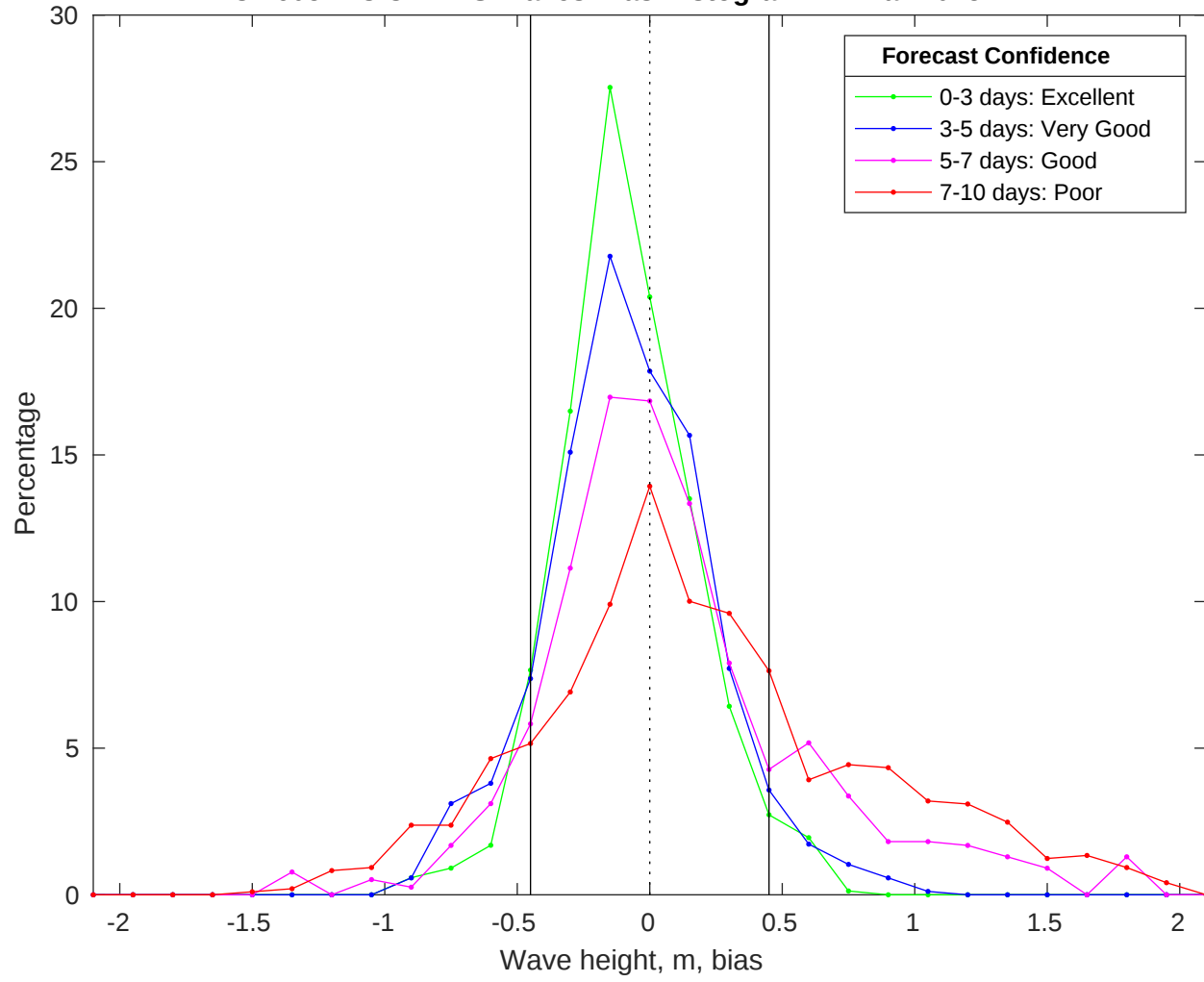
NDBC 46054 vs CMEMS Waves Bias Histogram: 21-Mar-2025
