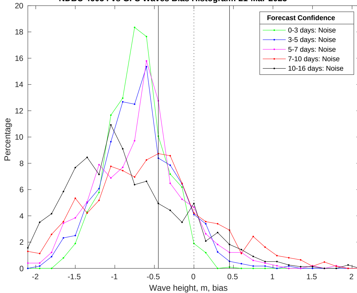
NDBC 46054 vs GFS Waves Bias Histogram: 21-Mar-2025
