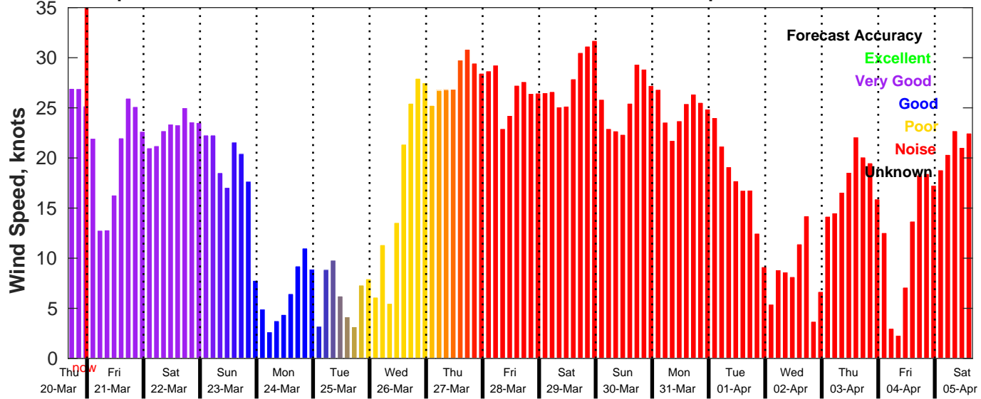
GFS Wind Speed Forecast for NDBC 46054 from 20-Mar-2025 16:00:00 to 05-Apr-2025 16:00:00
