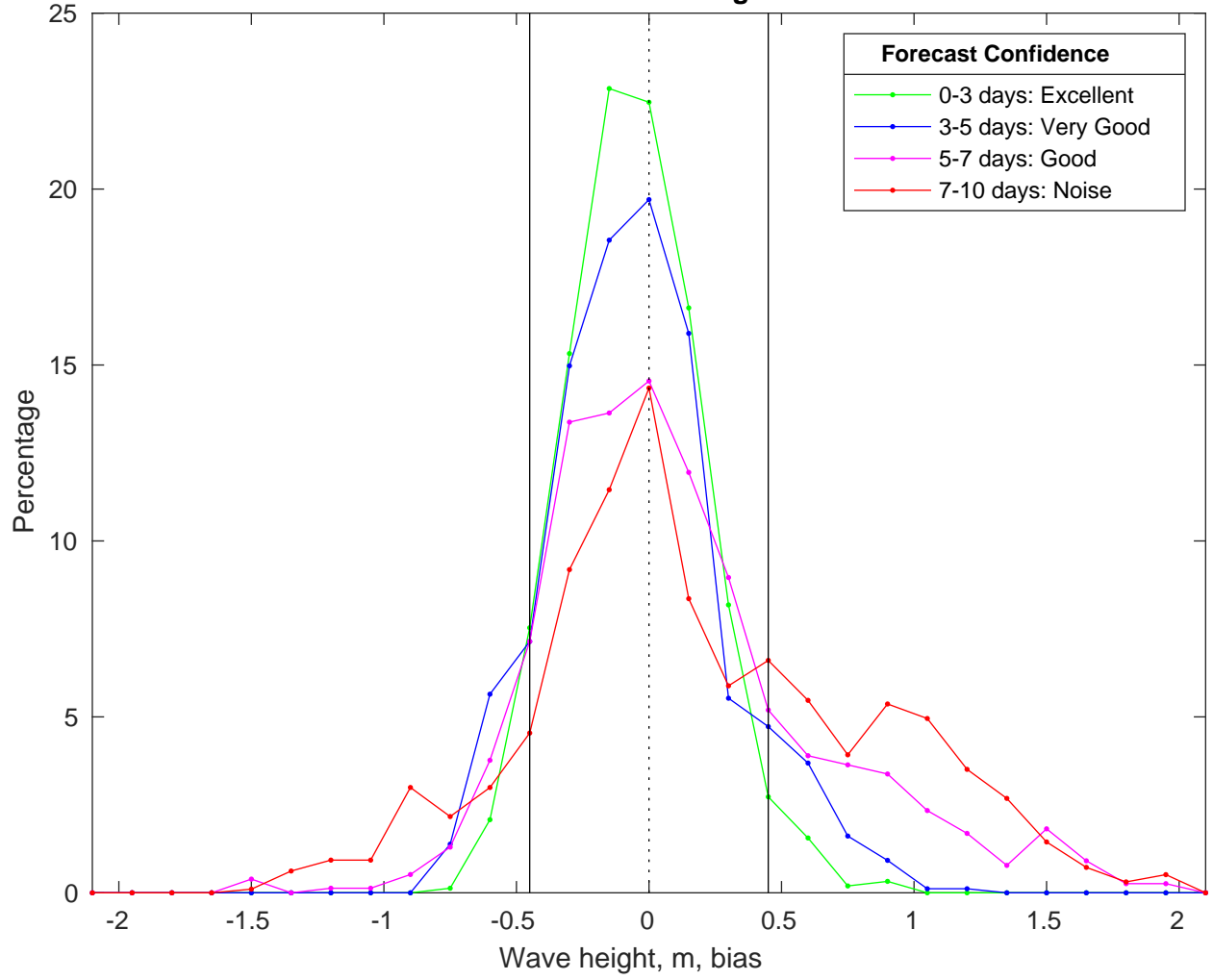
NDBC 46069 vs CMEMS Waves Bias Histogram: 21-Mar-2025
