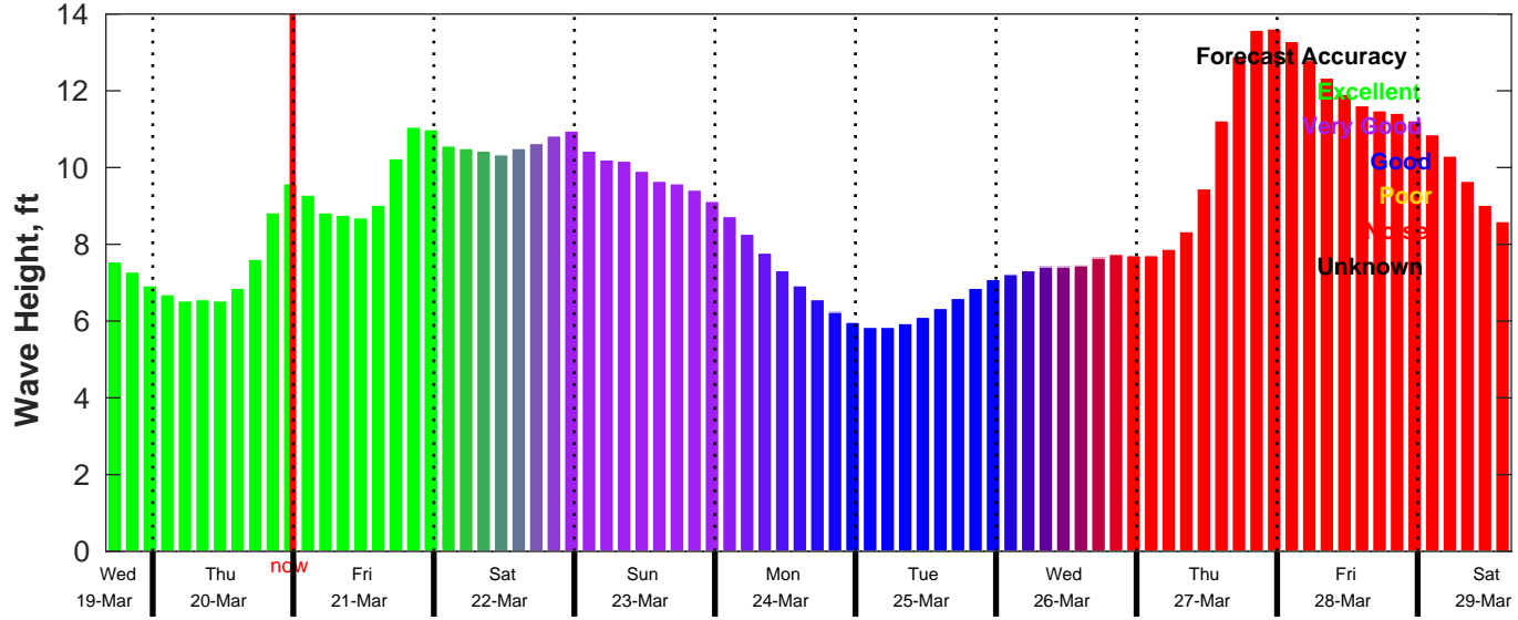
CMEMS Wave Forecast for NDBC 46069 from 19-Mar-2025 16:00:00 to 29-Mar-2025 16:00:00
