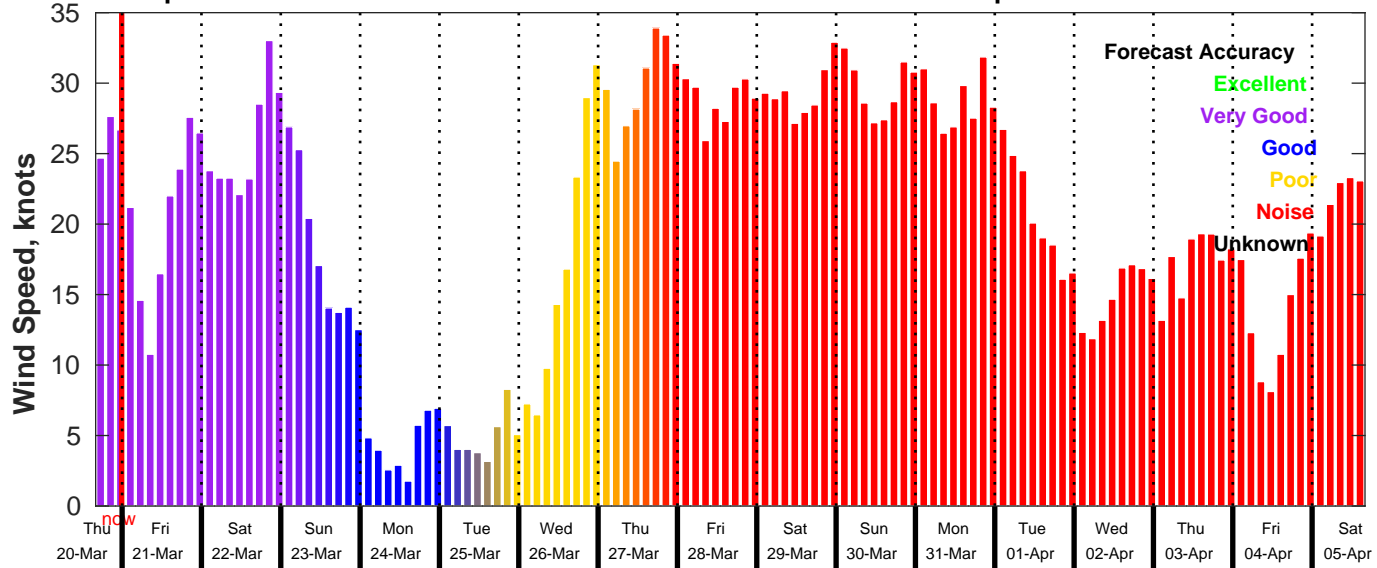
GFS Wind Speed Forecast for NDBC 46069 from 20-Mar-2025 16:00:00 to 05-Apr-2025 16:00:00
