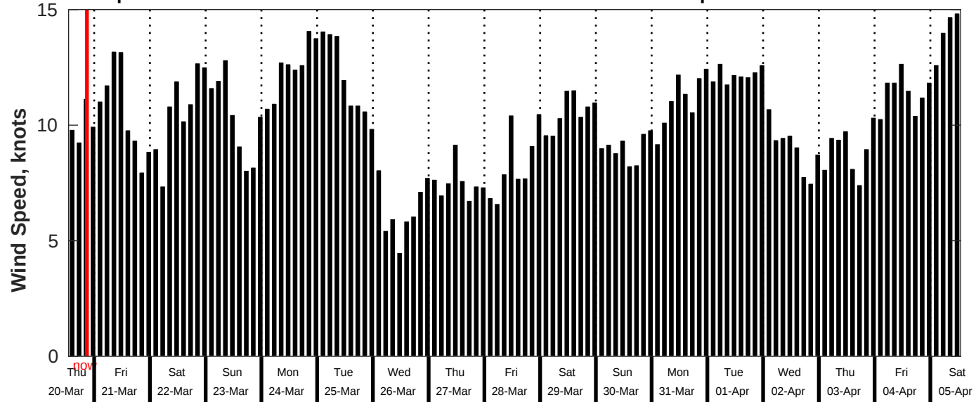
GFS Wind Speed Forecast for NDBC 51209 from 20-Mar-2025 13:00:00 to 05-Apr-2025 13:00:00
