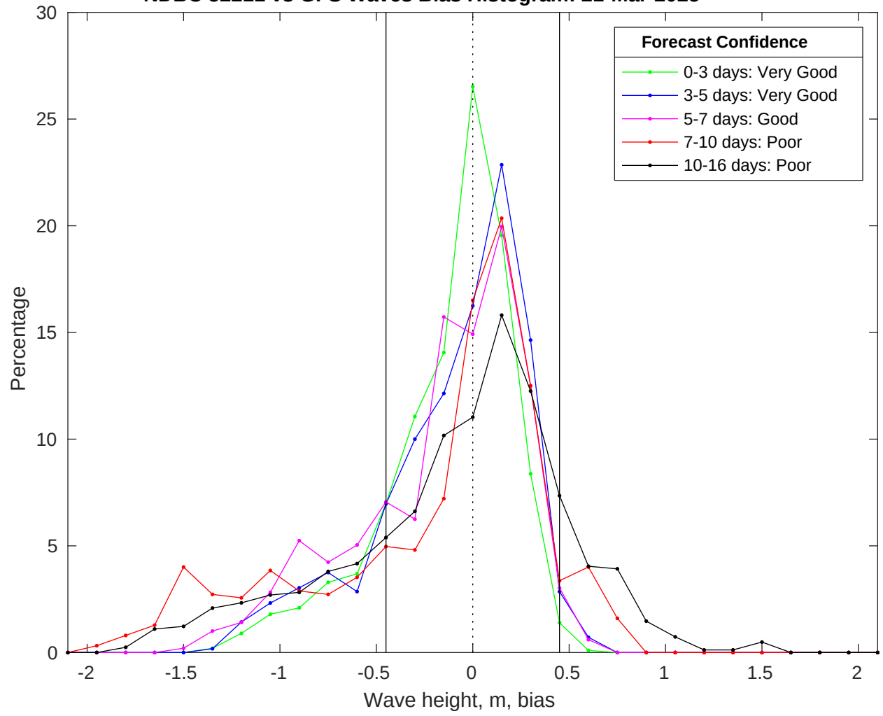
NDBC 52211 vs GFS Waves Bias Histogram: 21-Mar-2025
