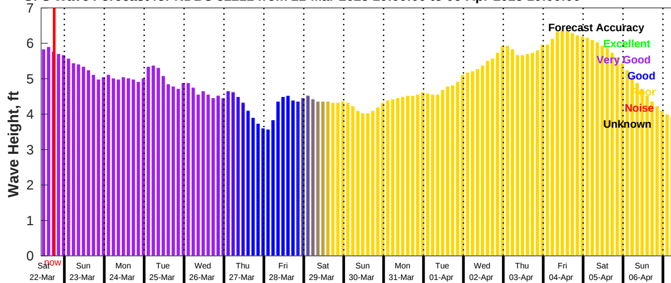
GFS Wave Forecast for NDBC 52211 from 21-Mar-2025 10:00:00 to 06-Apr-2025 10:00:00
