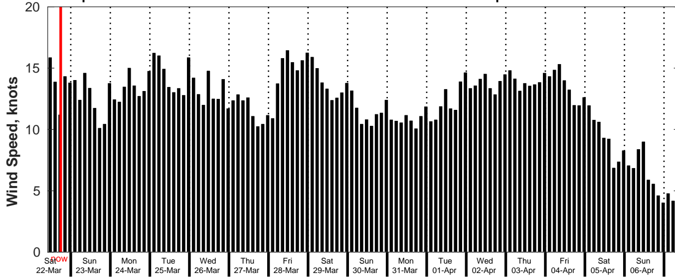
GFS Wind Speed Forecast for NDBC 52211 from 21-Mar-2025 10:00:00 to 06-Apr-2025 10:00:00
