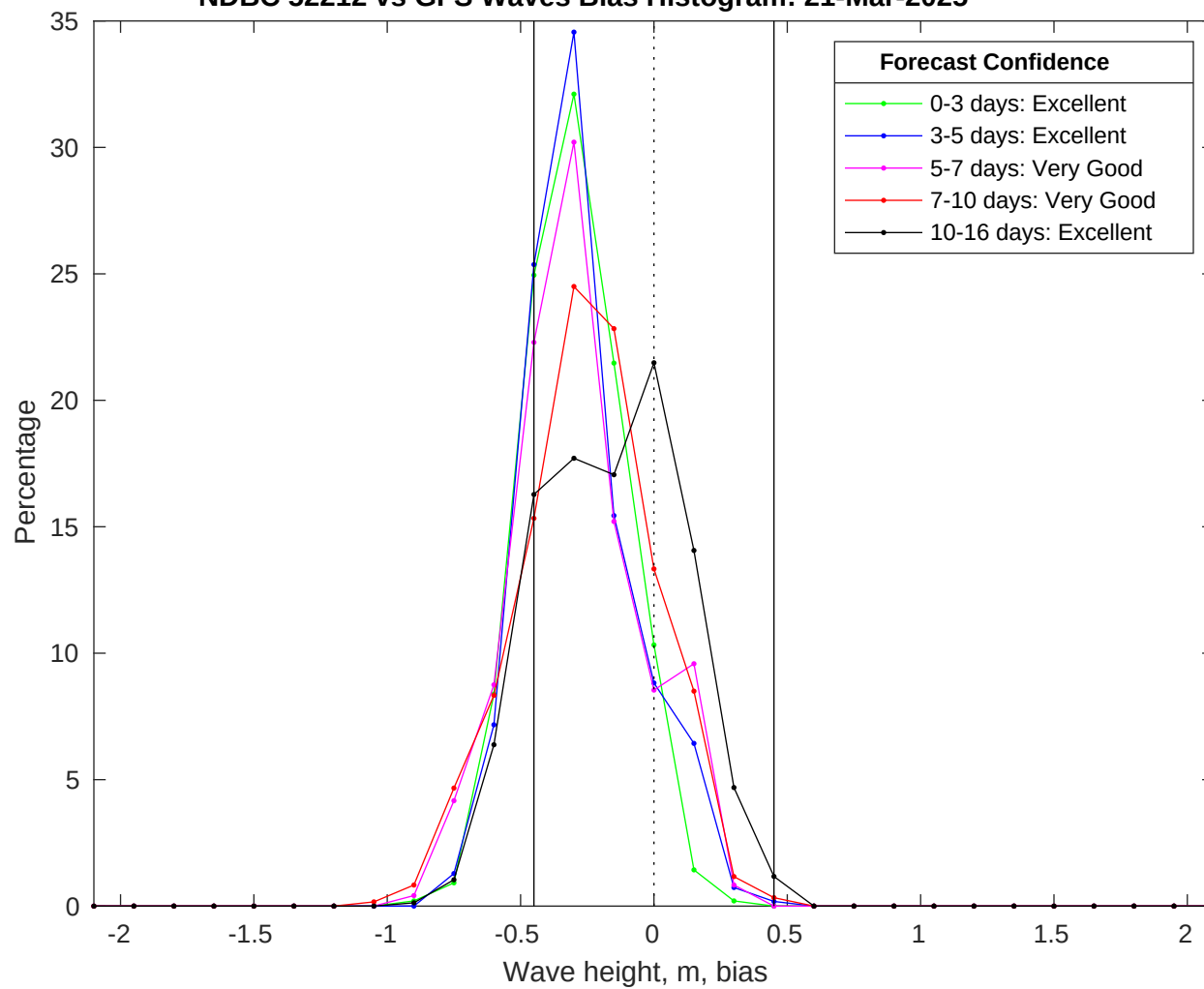
NDBC 52212 vs GFS Waves Bias Histogram: 21-Mar-2025
