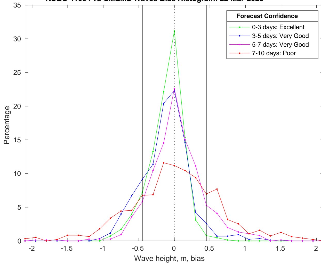
NDBC 41004 vs CMEMS Waves Bias Histogram: 22-Mar-2025
