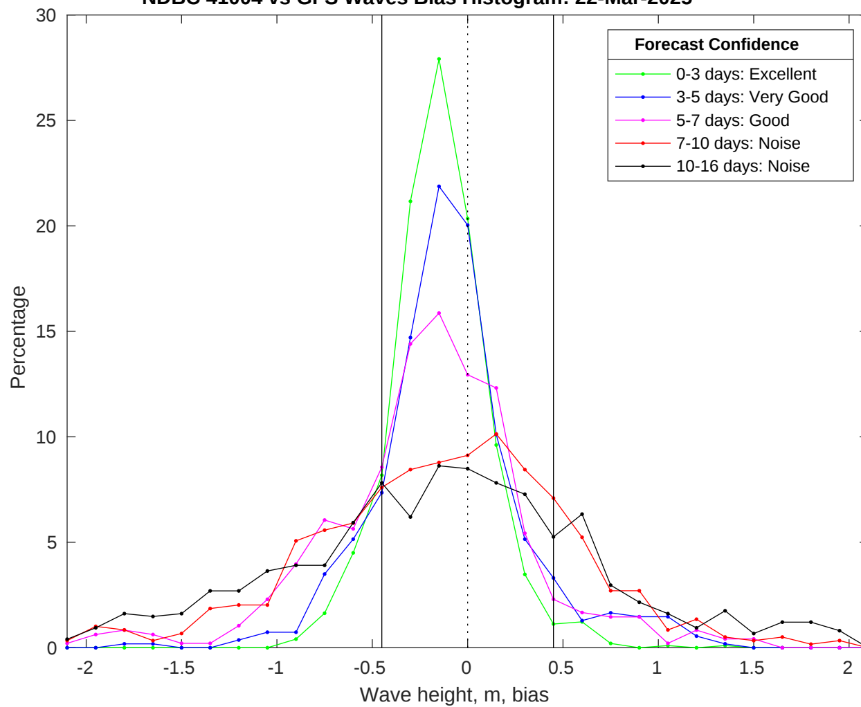
NDBC 41004 vs GFS Waves Bias Histogram: 22-Mar-2025
