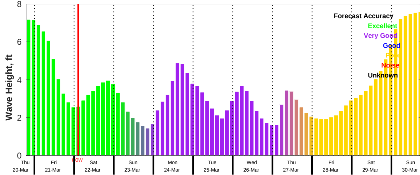
CMEMS Wave Forecast for NDBC 41004 from 20-Mar-2025 19:00:00 to 30-Mar-2025 19:00:00
