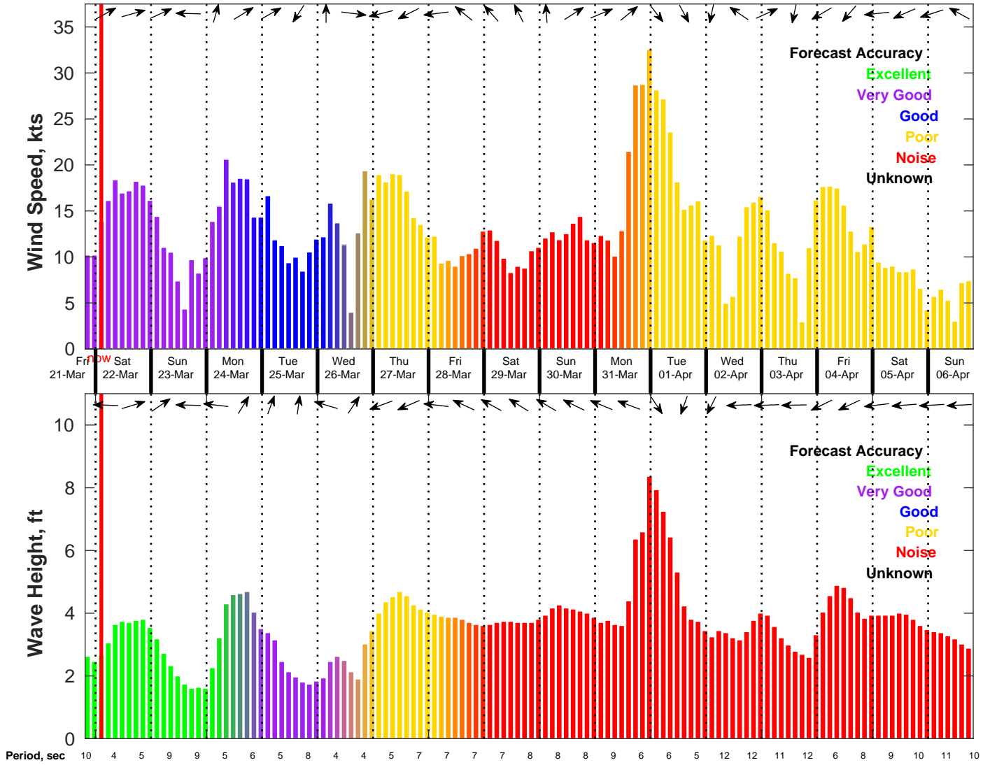
Wind & Wave Forecast for NDBC 41004 from 21-Mar-2025 19:00:00 to 06-Apr-2025 19:00:00
