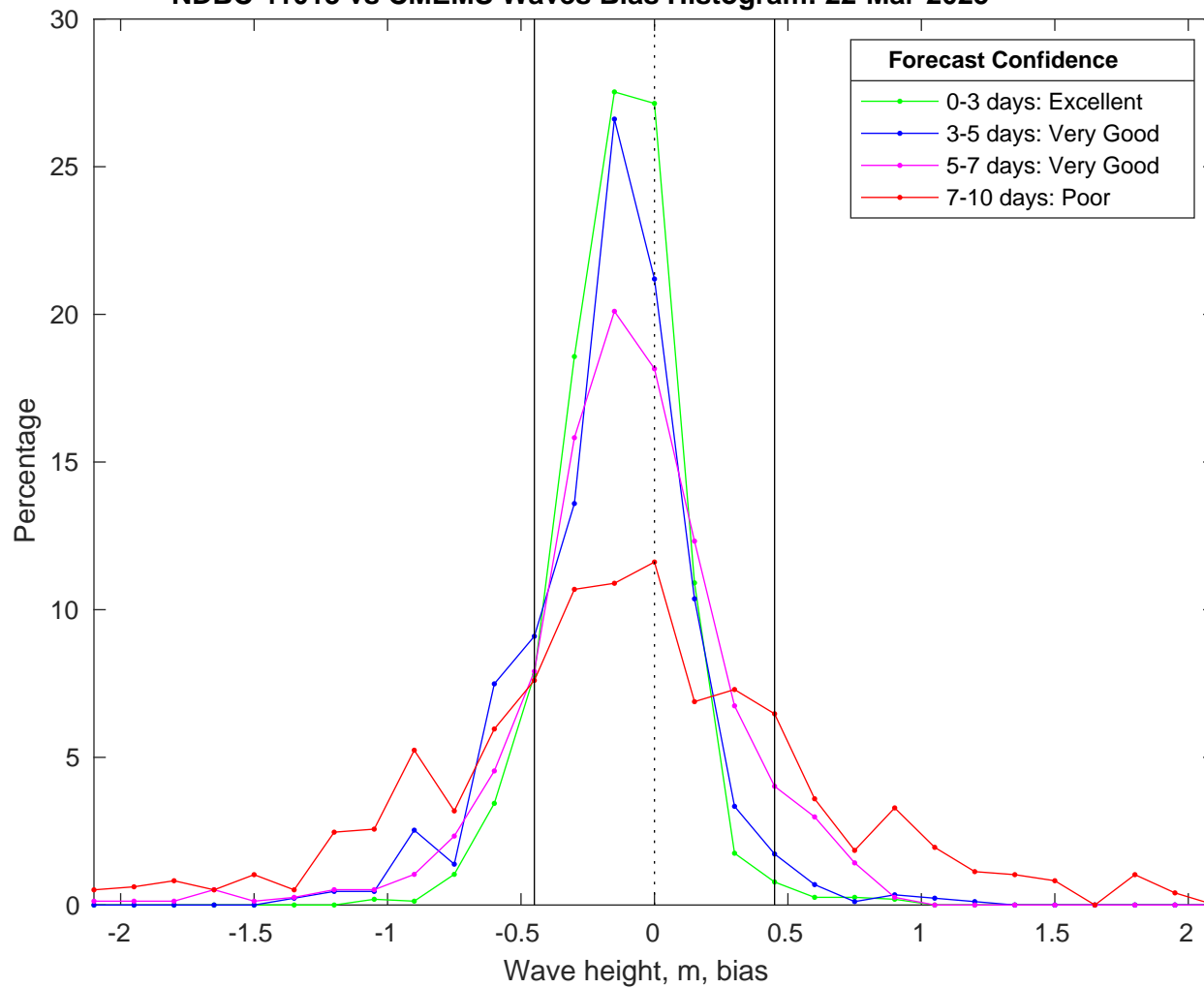
NDBC 41013 vs CMEMS Waves Bias Histogram: 22-Mar-2025
