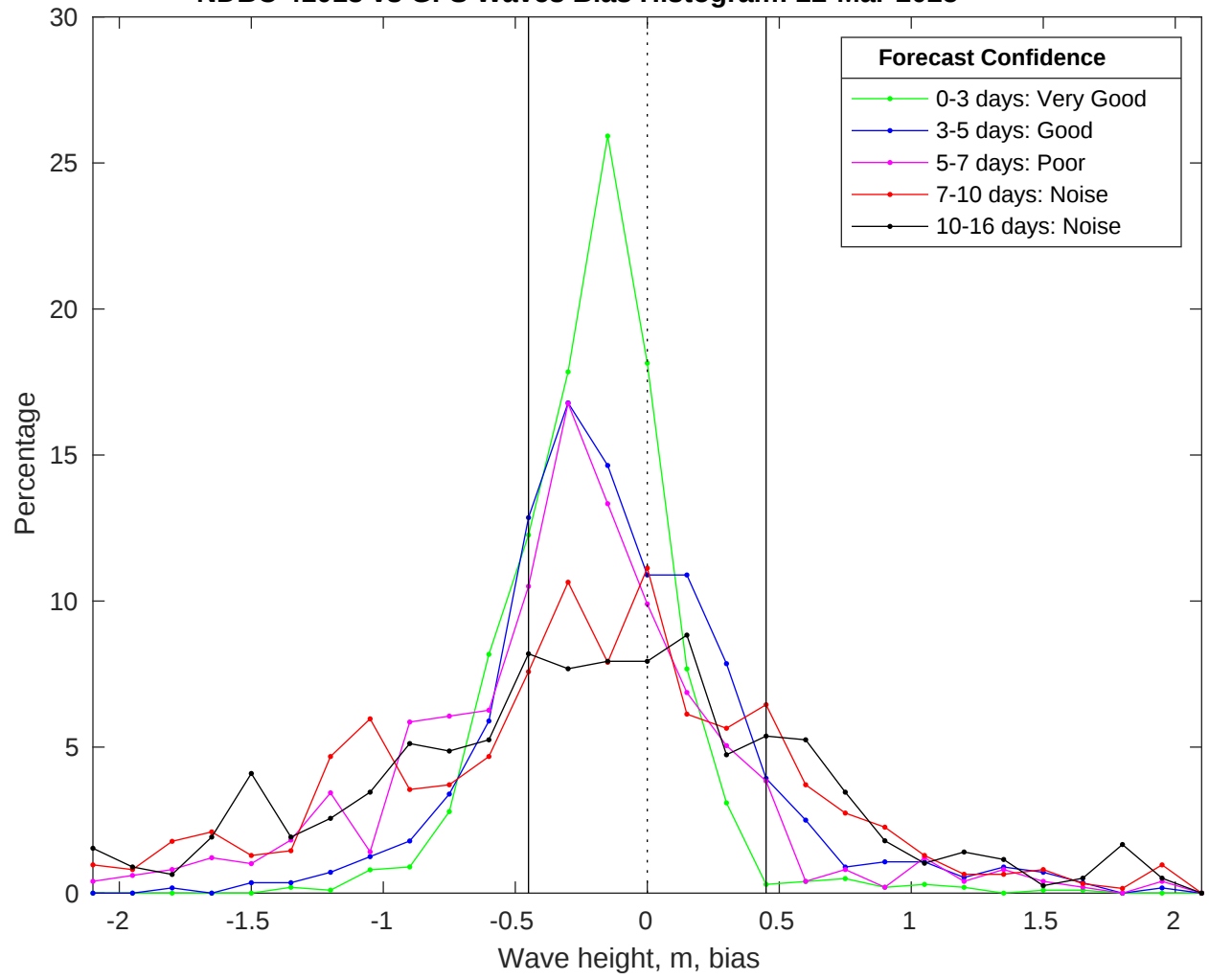
NDBC 41013 vs GFS Waves Bias Histogram: 22-Mar-2025
