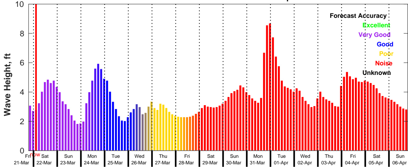
GFS Wave Forecast for NDBC 41013 from 21-Mar-2025 19:00:00 to 06-Apr-2025 19:00:00
