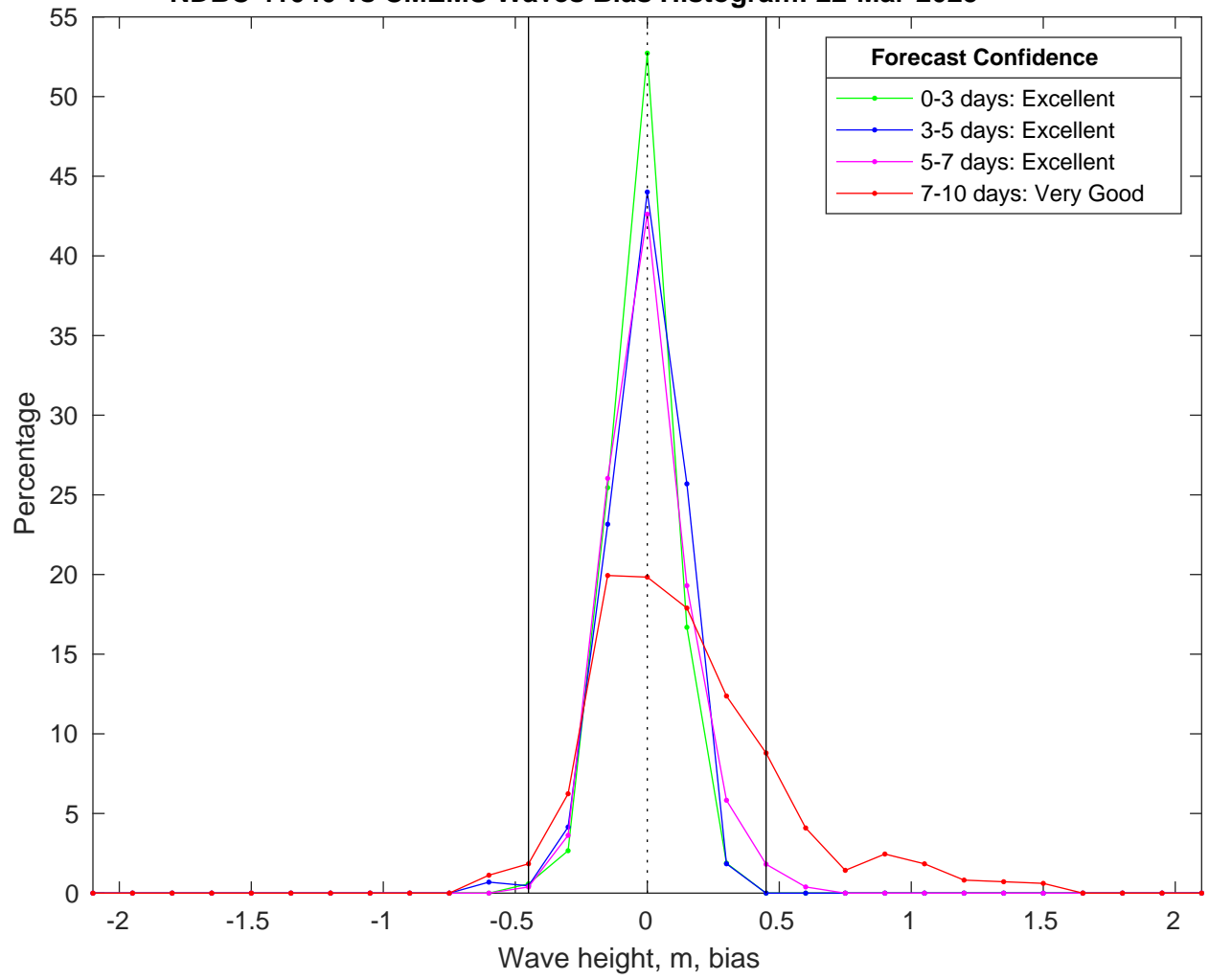
NDBC 41040 vs CMEMS Waves Bias Histogram: 22-Mar-2025
