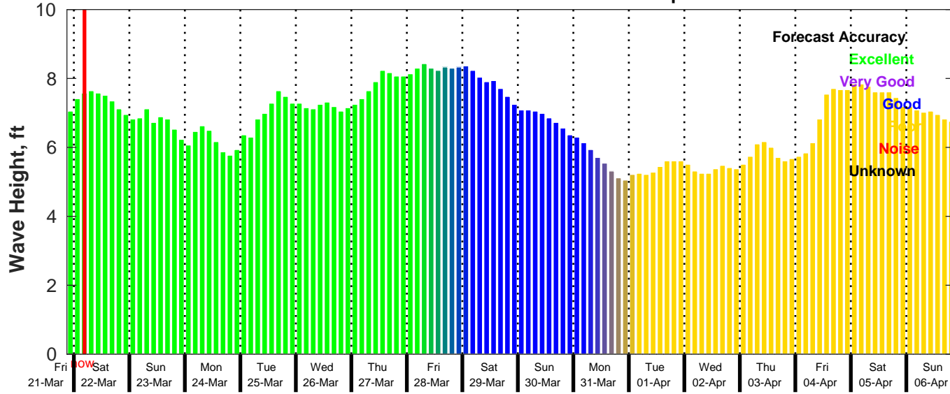
GFS Wave Forecast for NDBC 41040 from 21-Mar-2025 21:00:00 to 06-Apr-2025 21:00:00
