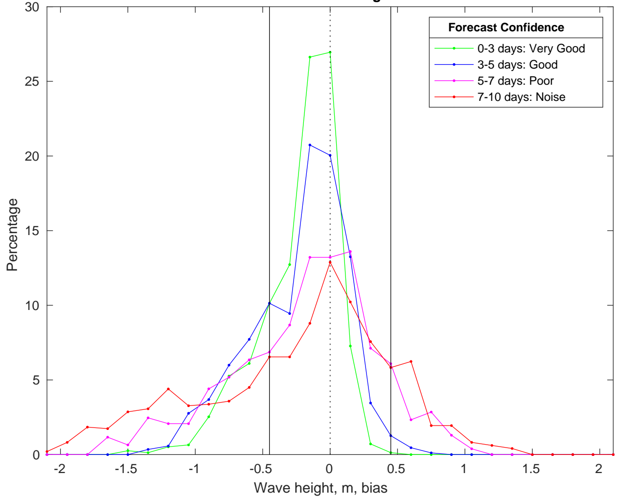
NDBC 42019 vs CMEMS Waves Bias Histogram: 22-Mar-2025
