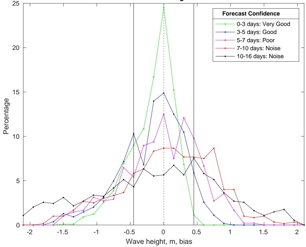
NDBC 42019 vs GFS Waves Bias Histogram: 22-Mar-2025
