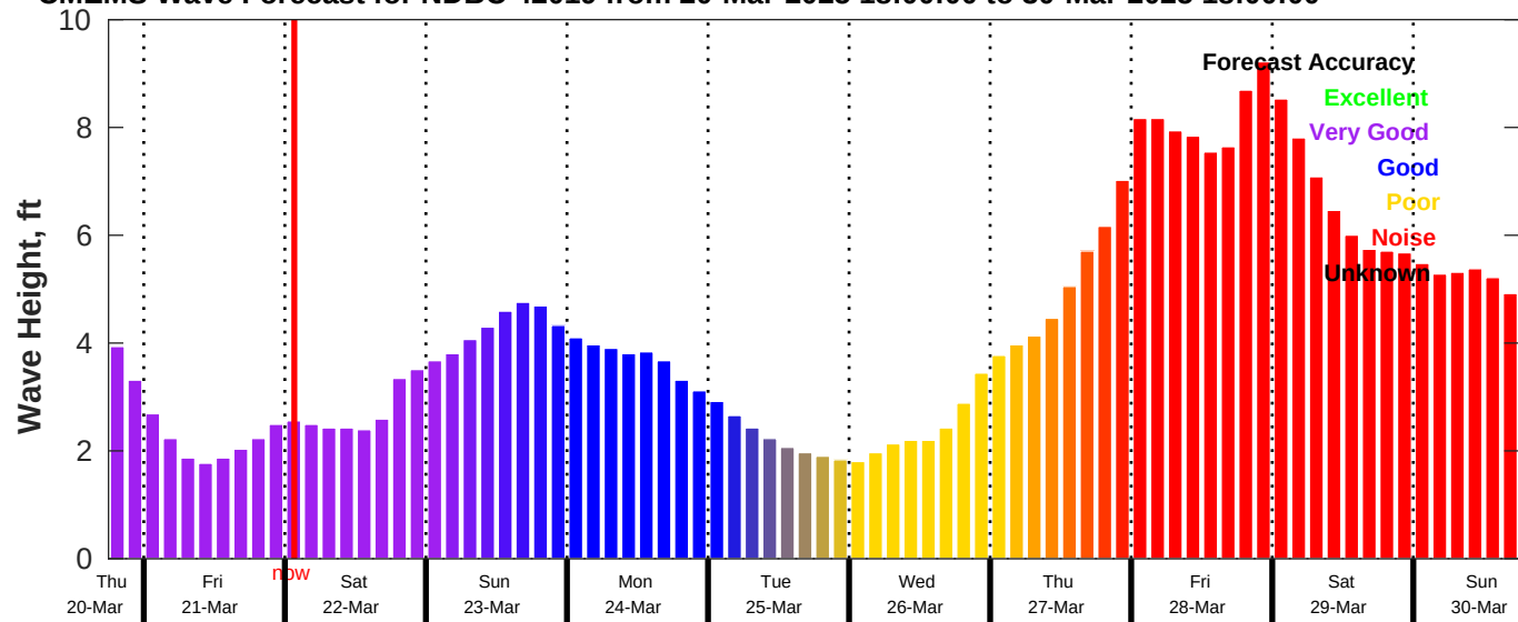
CMEMS Wave Forecast for NDBC 42019 from 20-Mar-2025 18:00:00 to 30-Mar-2025 18:00:00
