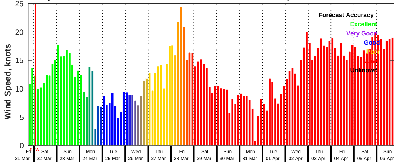
GFS Wind Speed Forecast for NDBC 42019 from 21-Mar-2025 18:00:00 to 06-Apr-2025 18:00:00
